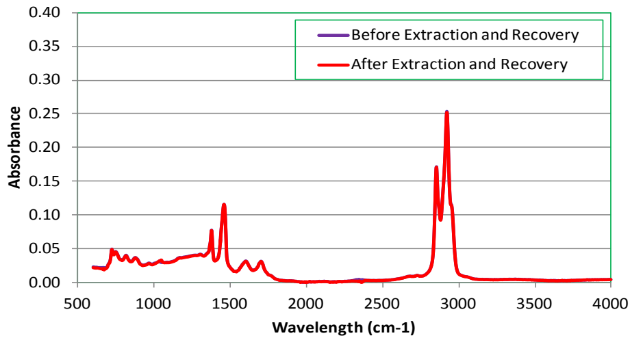
FTIR: Original Shingles Binder-before and after Extraction and Recovery
