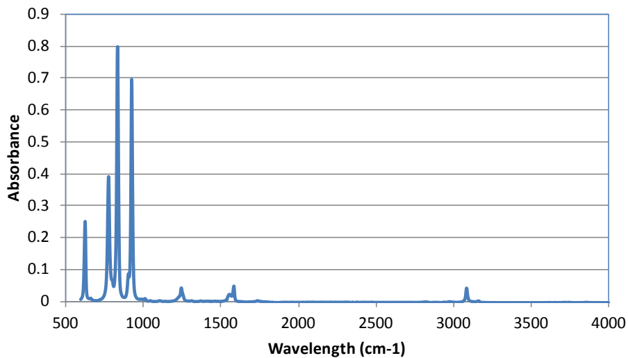
FTIR: Trichloroethylene
